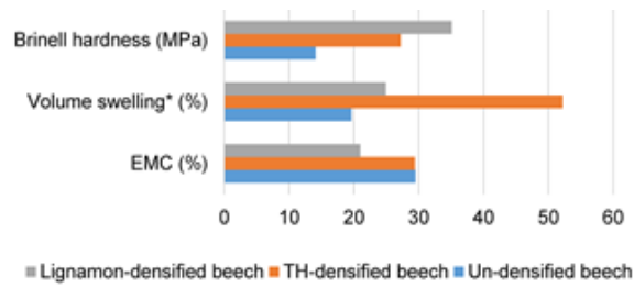
Figure 3. The Lignamon process compared to control and steamed-densified beech (based on Pařil et al. 2014)
