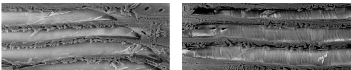
Figure 7. SEM images on radial sections of oak: before (left) and after (right) longitudinal compression (magnification 1000x) (images from Báder M.)
