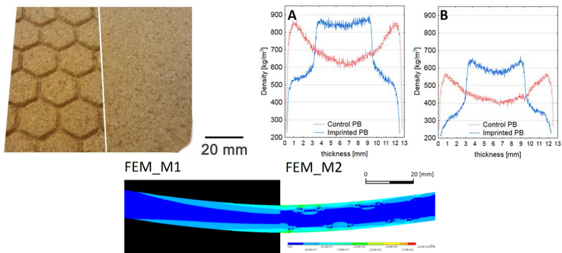
Figure 8. Surface of imprinted and control particleboards (top left), density profile of imprinted and control particleboards (top right) and calculated stress distribution in control (FEM_M1) and imprinted particleboard with veneered surface (FEM_M2) (Klímek et al. 2017)
