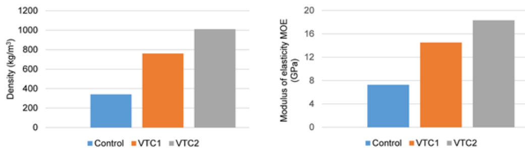
Figure 4. Densification of light-weight poplar wood by the VTC-process, i.e. heating and steaming in a closed-system at 170-200°C for about 7 min and compression. The compression ratio was 1:2.3 for control to VTC1 samples and 1:2.9 for the control to VTC2 samples (based on Rademacher et al. 2014)
