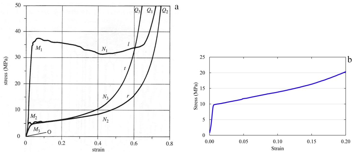
Figure 2. Stress-strain curves of samples of poplar (a) of dimensions 25x25x5 mm 3 subjected to compression in the l, r, t directions under controlled displacement at a rate of 1 mm/min (Navi and Sandberg 2012), and oak (b) subjected to controlled compression in the longitudinal direction (based on Báder and Németh 2018)
