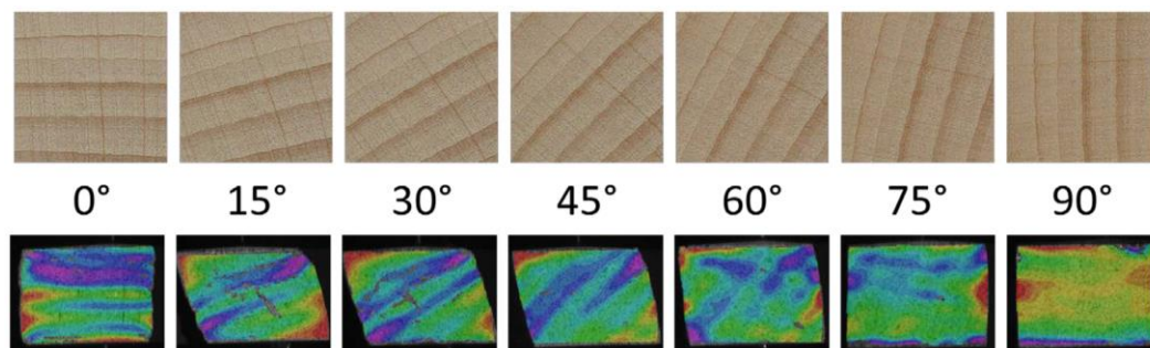
Figure 1. Densification of beech with different annual ring orientations in the cross section and Digital Image Correlation (DIC) showing the strain at 26% compression (blue colour: high strain; red colour: low strain) (Rousek 2014)
