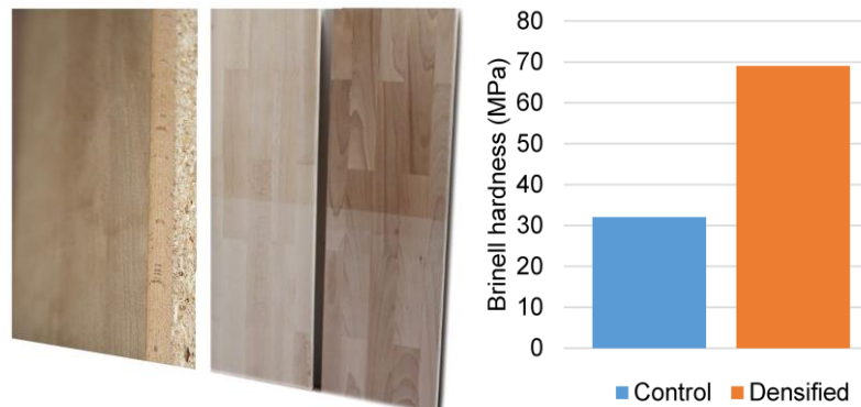
Figure 6. A layered flooring panel (left) with densified beech as top surface (on the right of the center image), an undensified beech (on the left of the center image) and Brinell hardness values (right) (based on Dömény et al. 2014)
