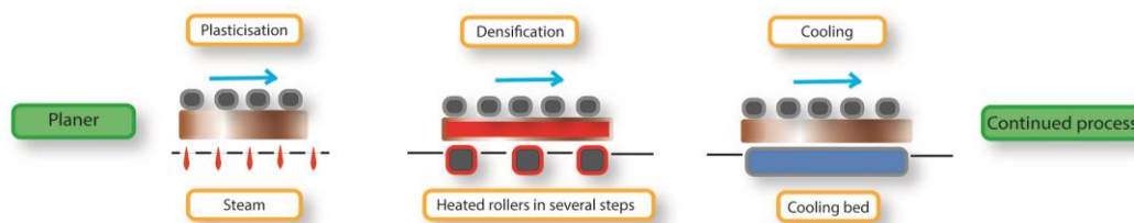
Figure 5. Schematic illustration of a continuous surface densification process (from Sandberg et al. 2017)
