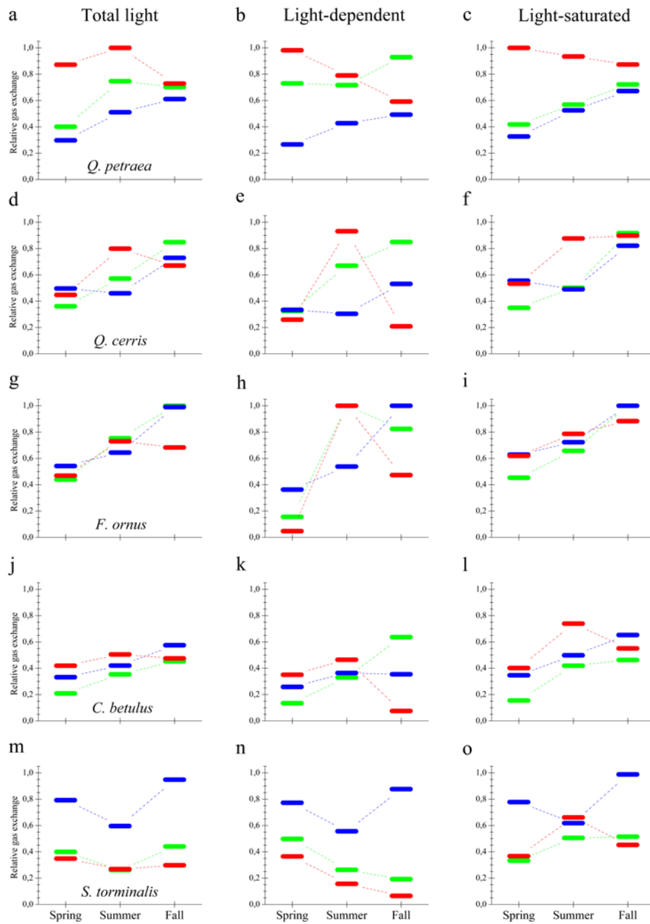
Figure 2. Functional fingerprints of the study species in canopy gaps along the light response ranges (total to light saturated) with assimilation (green), stomatal conductance (blue) and intrinsic water use efficiency (red). Relative gas exchange refers to standardized mean considering all cases of the given parameter.
