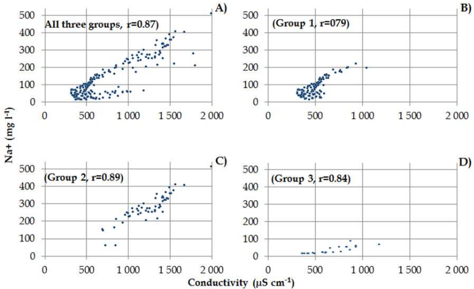
Fig. 9. x-y scatterplot showing the relationship between Na + and conductivity for all the groups (A), group 1 (B), group 2 (C), and group 3 (D)
