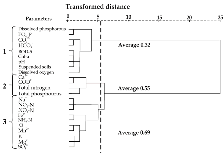
Fig. 5. Dendrogram of Wilks' lambda quotients
